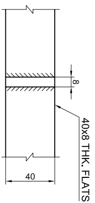
DETAIL-X SCALE-1:2
